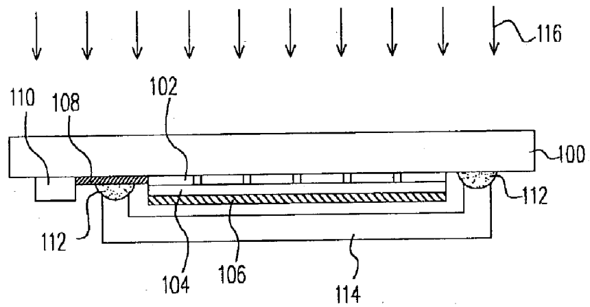
FIG. 2 (PRIOR ART)
